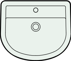
Quantum Round 600mm Standard Basin W600 x D480mm Full Pedestal H830mm
