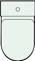
Quantum Square Close Coupled WC W360 x D650 x H825mm
